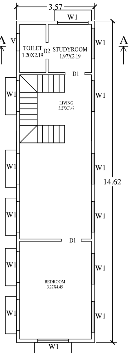
PROPOSED SECOND FLOOR PLAN
